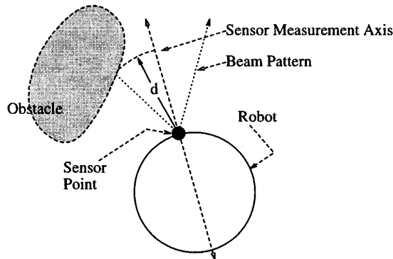
Fig. 2. Simplified Distance Measurement Sensor Model
