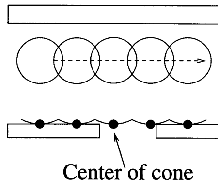
Fig. 6. Passing a line through the centers of the cones gives the robot the impression there is one wall.
