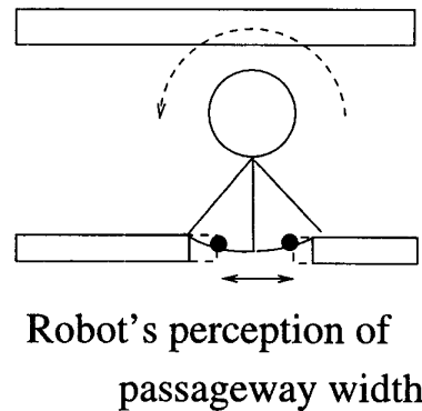
Fig. 5. Center of cone makes the passageway seem narrower
