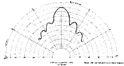
Fig. 1. Beam pattern for the Polaroid transducer installed on many mobile robots.
