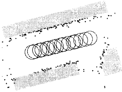
Fig. 7. Centerline method was used. The points correspond to the center of arcs from real sonar data and the light grey obstacles were drawn for the sake of display. The actual obstacles were walls in the lab.
